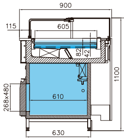
VMINVT-VDB UV 3M2 ventilada total total ventilated
