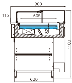
VMINVS-VDB UV 3M2 ventilada superior upper ventilated
