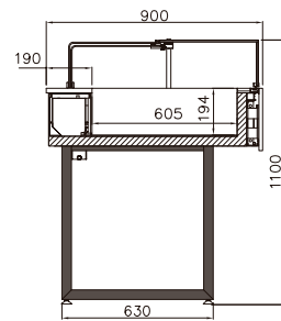
VMINPD-VDB UV padaria bakery
