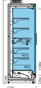
MF2 700 P CP SG 3M1/3M2 carne, charcutaria laticínios meat, delicatessen dairy products
