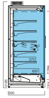
MF2 900 P CP SG 3M1/3M2 carne, charcutaria laticínios meat, delicatessen dairy products
