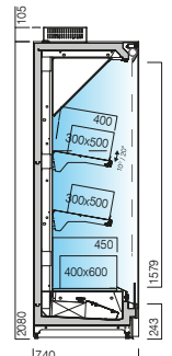
MF2 700 PF CC SG 3H1 frutas, legumes e flores produce and flowers
