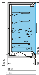
MF2 900 P CP CG 3M1/3M2 carne, charcutaria laticínios meat, delicatessen dairy products
