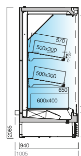
MF2 900 PF CC CG 3H1 frutas, legumes e flores produce and flowers
