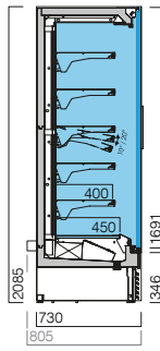
MF2 700 P CP CG 3M1/3M2 carne, charcutaria laticínios meat, delicatessen dairy products
