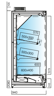
MF2 900 PF CC SG 3H1 frutas, legumes e flores produce and flowers
