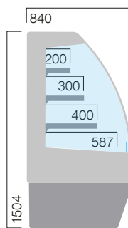
SMVCT 4N H15 3M2 refrigerado ventilado chilled ventilated +3°... +6° C dim. 625 | 937 | 1250 | 1875
