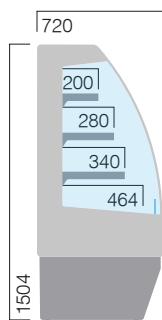
SMVCTS H15 3M2 refrigerado ventilado chilled ventilated +3°... +6° C dim. 625 | 937 | 1250 | 1875
